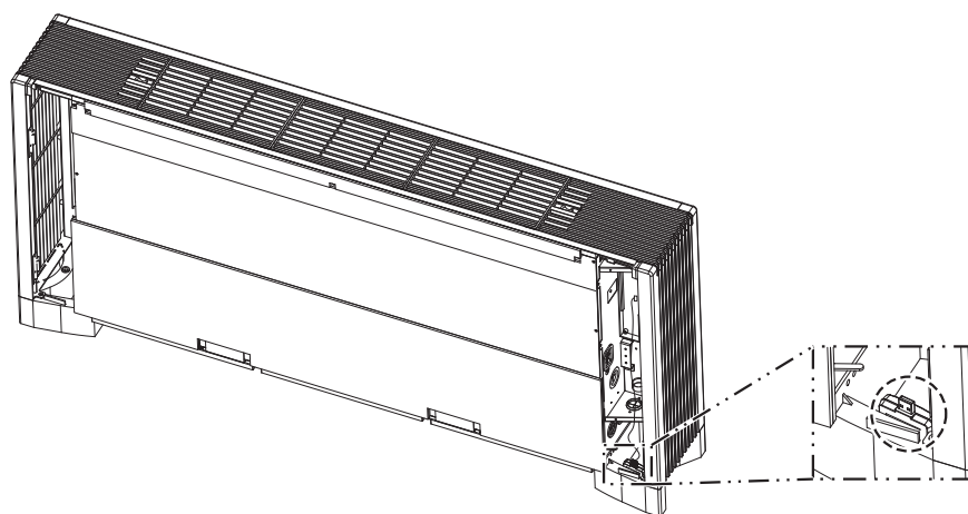
<Installation Example>
