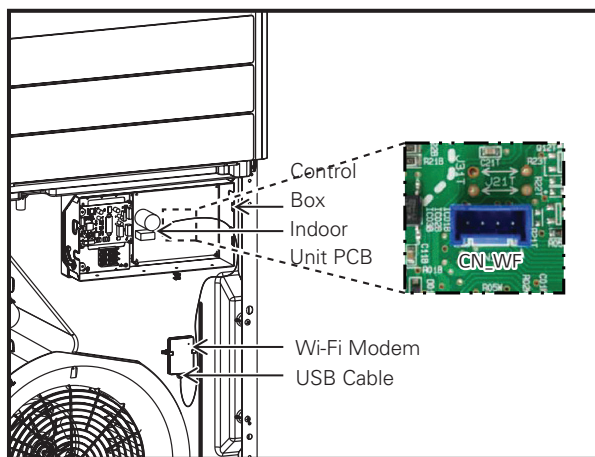
Installation Plan 1
